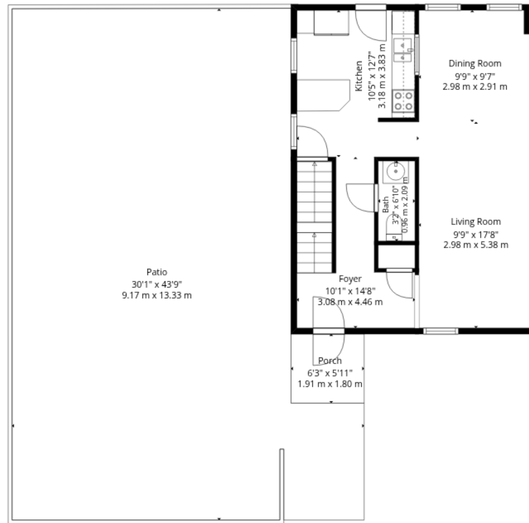
1st Floor
